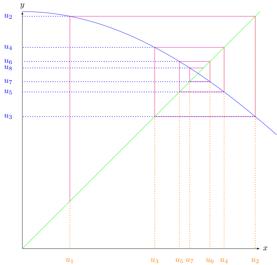
Figure 1: f(x) = \cos(x)
